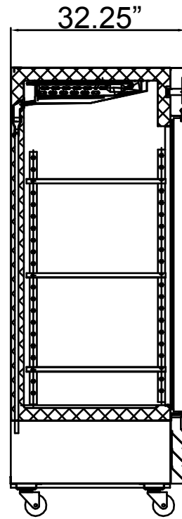
SECTION VIEW
